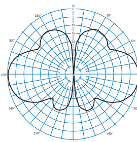
Typical E-Plane response for CD920
