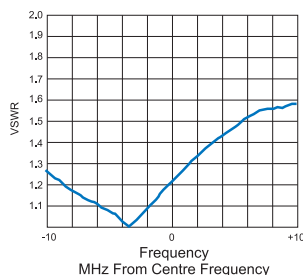
Typical full band VSWR Response (CD920)
